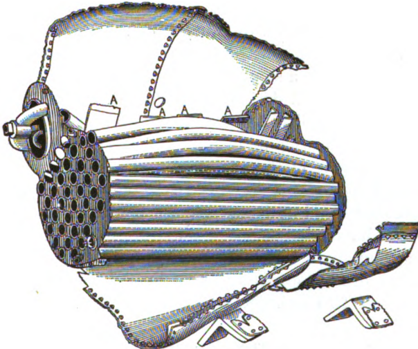
FIG. 135.—DEFECTIVE FORM.
